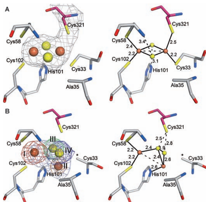
Figure 2. A) The \text{Fe}_2\text{S}_2 complex with its classical cluster depicted as spheres and IscS Cys321, and the corresponding omit electron density map (left) and bond distances (right). B) The partially oxidized complex with the \text{Fe}_2\text{S-S} atoms (I–IV) depicted as spheres, their corresponding omit map peaks, and the global omit map (light blue, left). The \mu_2\text{-}\eta^3 sulfido ligation has been observed in a model compound [9] (see Figure S5 in the Supporting Information). The maps are contoured at the 3 \sigma level. The -S(H) (indicated by a star) from Cys33 is not visible in the map due to disorder and, consequently, has not been included in the model. Carbon atoms are colored gray and pink in IscU and IscS, respectively.
