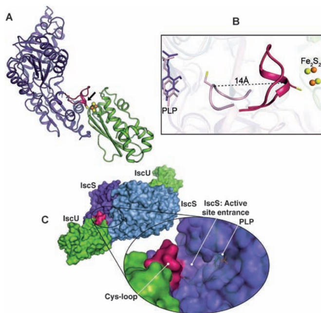
Figure 1. \text{Af}(\text{Fe}_2\text{S}_2\text{-(IscS-IscU}^{\text{D35A}}\text{)})_2 complex structure. A) Ribbon representation of the heterodimer \text{Fe}_2\text{S}_2\text{-(IscS-IscU}^{\text{D35A}}\text{)} . IscS and IscU D35A are represented in purple and green, respectively. The black arrow points at the Cys loop depicted in pink. B) Different conformations for the Cys loop in the IscU D35A -bound \text{AfIscS} (pink, this work) and in Synechocystis SufS (light pink). [17] C) Surface representation of the complex. The two IscS molecules are depicted in purple and gray-blue and the two IscU D35A molecules in green; the IscS Cys loop is shown in pink. Close-up view: the semitransparent IscS surface highlights the PLP position, located deep inside a tunnel. The Cys loop does not occlude this tunnel, which allows for cysteine diffusion to the IscS active site and Cys-loop movements during the cluster assembly process without complex dissociation. This view is rotated by 180° relative to (A).
