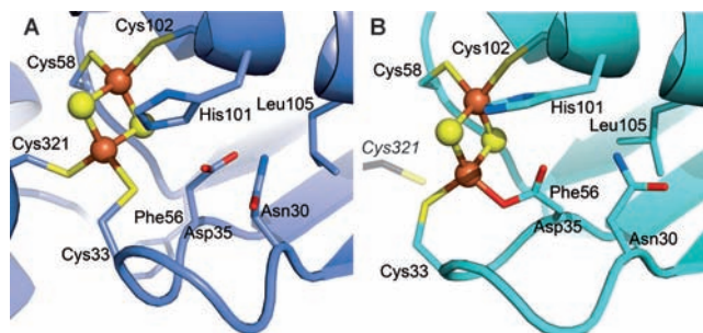
Figure 3. Models from QM/MM calculations. Geometry-optimized structure of A) the Af(Fe_2S_2-(IscS-IscU))_2 complex and B) a model of AfFe_2S_2-IscU where sampling of loop 30–35 was performed to evaluate whether Cys33 and Asp35 could coordinate the cluster. Cys33 replaces IscS Cys321 (see the Supporting Information for details).
